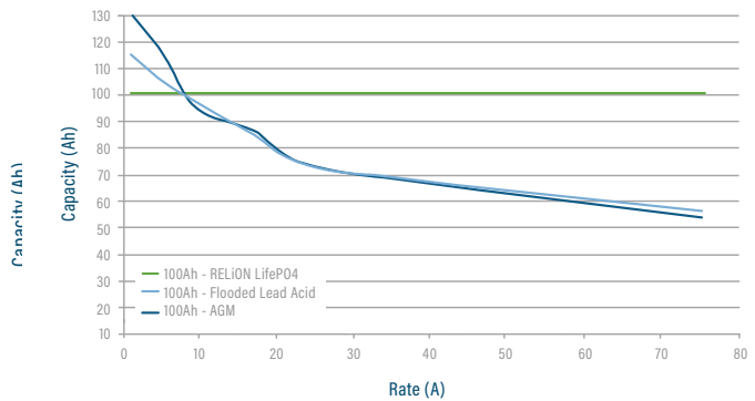
CAPACITY OF RELiON LiFePO4 vs. LEAD ACID at VARIOUS RATES OF DISCHARGE
