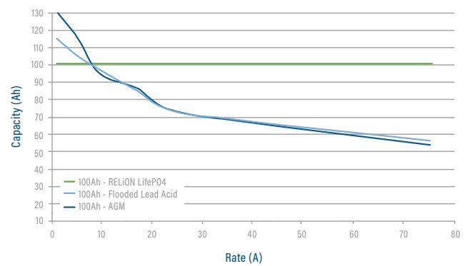
CAPACITY OF RELIION LiFePO4 vs. LEAD ACID at VARIOUS RATES OF DISCHARGE
